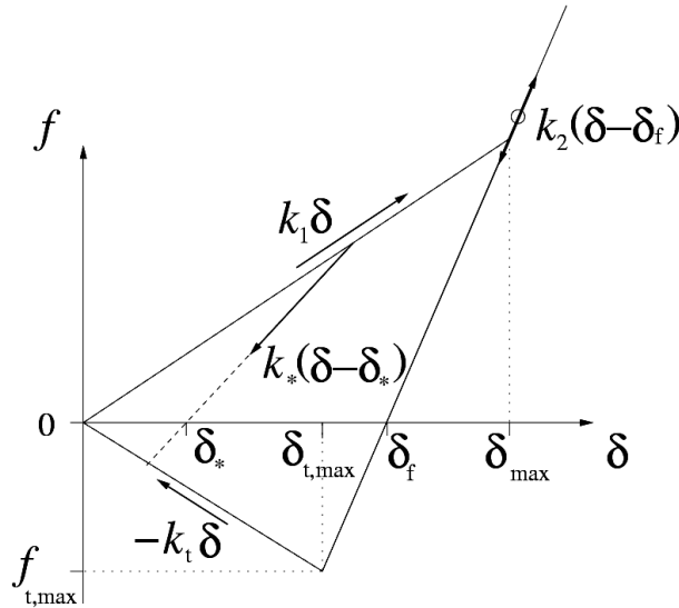
Fig. 2: Particle contact model plotted as force-displacement relation [11][23], with d for contact positive, and repulsion and attraction forces positive and negative, respectively.
