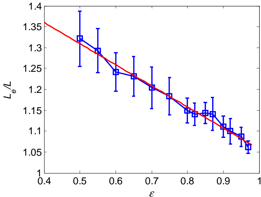
Figure 2: Variation of tortuosity L_e/L , as a function of porosity. The solid red line shows the linear best (least square) fit and the error bars indicate the standard deviations from 8 equal mass flux streamlines.
