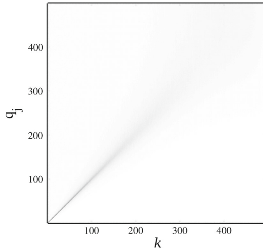
Fig. 11 Absolute values of the components of \mathbf{q} (see text) for varied input waveforms \mathbf{u}_0 , which for increasing k along the horizontal axis become wider spread out (lower shades of gray) across the eigenmodes. Results are produced for an ensemble of 200 chains of N = 500 particles with \xi = 0.5
