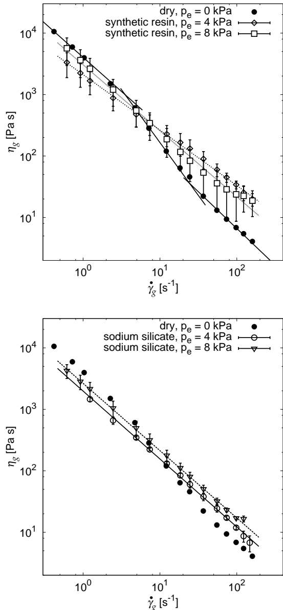
Fig. 2: Apparent shear viscosity \eta_g(\dot{\gamma}_g) for core shooting material made of F35 and synthetic resin binder with m_{SR}/m_F = 0.01 (top), and made of F35 and sodium silicate binder with m_{SS}/m_F = 0.02 (bottom); error bars indicate the standard deviation of the experimental data. Results of dry F35 are also given for comparison, performed with smaller gap b . Measurements are made with different external pressure levels p_e . Continuous and dashed lines indicate the scaling between \eta_g and \dot{\gamma}_g , obtained from least square fits of Eq. (2) to the wet data, for 0.4\text{ s}^{-1} < \dot{\gamma}_g < 200\text{ s}^{-1} .
