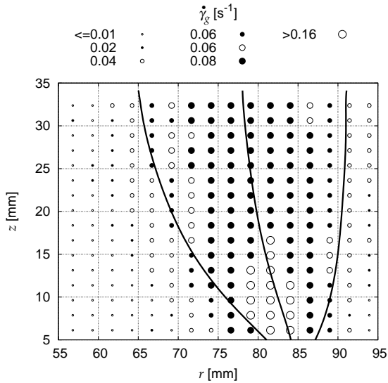
Fig. 9: Strain rate \dot{\gamma} as function of radial and vertical position within the rheometer gap. As in Fig. 8, different symbol sizes indicate the magnitude of \dot{\gamma} . The lines indicate the center location R_c (middle line) and the width W of the shear bands (outer lines), as obtained from the fit function Eq. (19).
