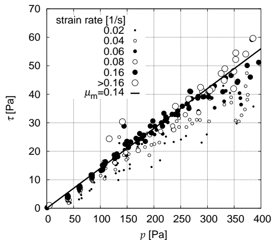
Fig. 8: Local shear stress |\tau| plotted against local pressure p . Different symbol sizes indicate the magnitude of the strain rate \dot{\gamma} at different locations within the rheometer gap, with \dot{\gamma} given in the inset in units of s^{-1} ; larger symbols correspond also to larger \dot{\gamma} . The solid line represents the function |\tau| = \mu_m p , with the macroscopic friction coefficient \mu_m = 0.14 .
