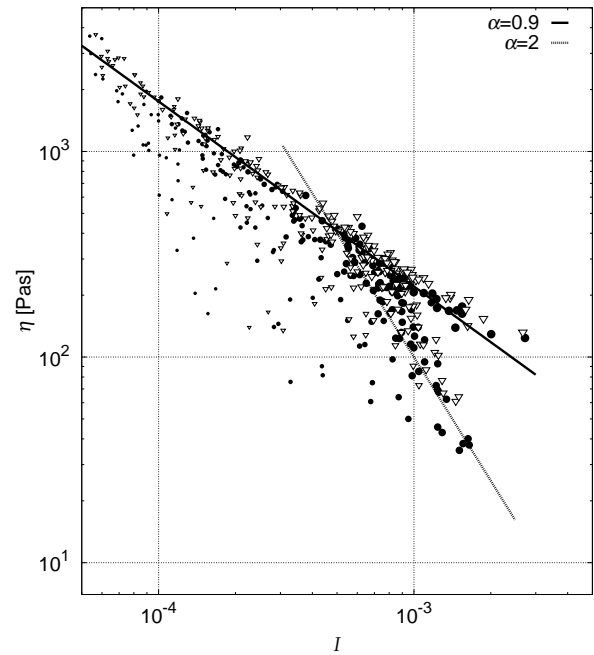
Fig. 12: Apparent shear viscosity \eta(I) from the DEM simulations. Different symbols indicate results from dry ( \bullet ) and wet material (open symbols). The wet material contains liquid bridges with (top) \theta = 10^\circ ( \triangle ) and (bottom) \theta = 20^\circ ( \nabla ), whereas V_b = 42 nl is constant in all cases. The magnitude of the strain rate \dot{\gamma} is indicated by the size of the symbols similar as in Fig. 8.
