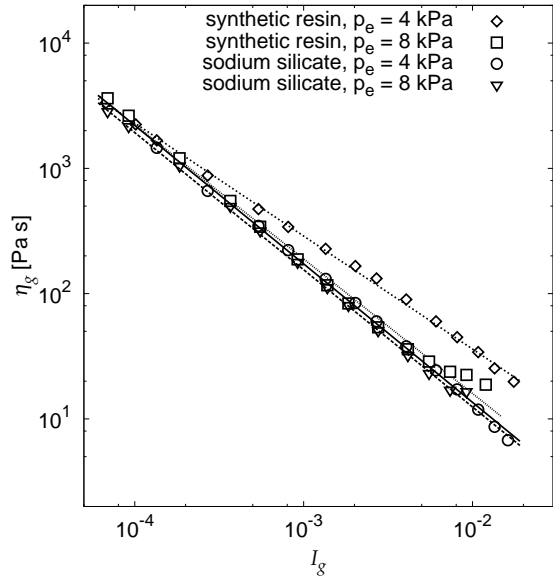
Fig. 3: Apparent shear viscosity as a function of dimensionless shear rate for the two core shooting materials and the two external pressure levels p_e of Fig. 2. Continuous and dashed lines indicate the scaling \eta_g \sim I_g^{-\alpha} , with \alpha from table 1.
