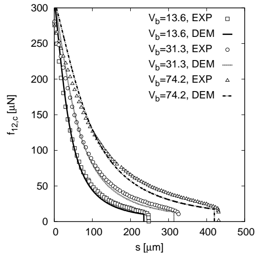
Fig. 6: Forces in a capillary bridge with contact angle \theta = 0^\circ between two equal-sized particles; lines indicate results of the DEM simulation, points give the experimental data of Willett et al. [15]. Liquid bridge volumes V_b are given in nano-liters ( 10^{-9}\text{l}=\text{nl} ).
