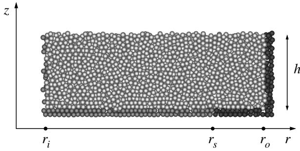
Fig. 7: Setup of the numerical rheometer, light gray: sheared granular material, medium gray: static, inner part of the shear cell, dark gray: rotating, outer part of the shear cell (the medium and dark gray particles are part of the rough walls of the shear cell and thus displayed as particles).
