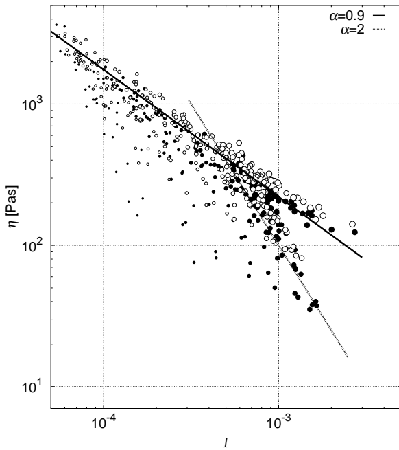
Fig. 11: Local shear viscosity \eta(I) from the DEM simulations. Different symbols indicate results from dry ( \bullet ) and wet material (open symbols). The wet material contains liquid bridges with (top) V_b = 4.2 nl ( \square ) and (bottom) V_b = 42 nl ( \circ ), whereas \theta = 0^\circ is the same for both cases. The magnitude of the local strain rate \dot{\gamma} is indicated by the size of the symbols similar as in Fig. 8.
